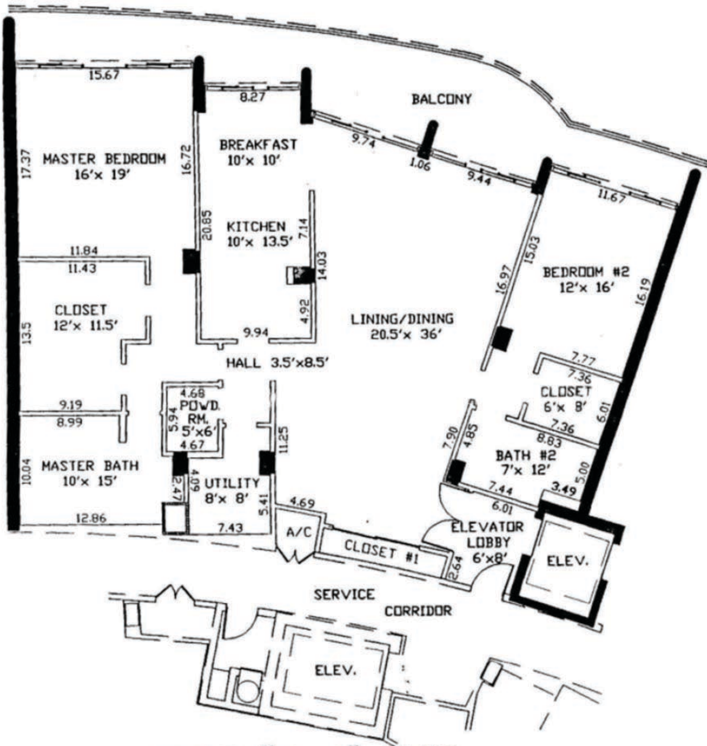
TYPE "S-4" UNIT UNIT S-404 THRU S-1704
