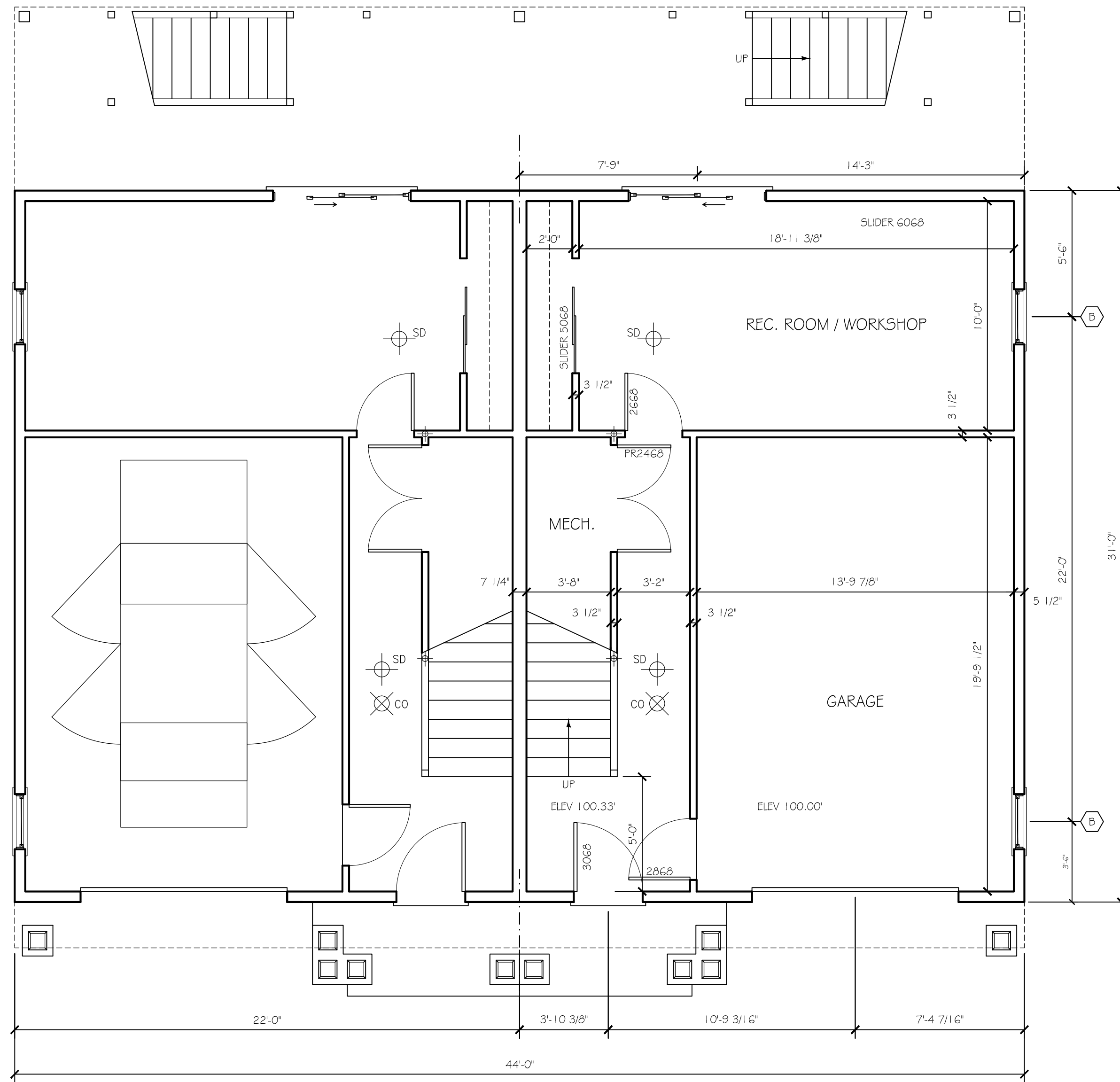
1 Garden Level Plan Scale: 1/4"=1'-0"
